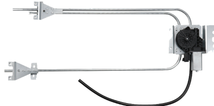
WINDOW REGULATOR (LH) (CASCADIA, CORONADO)
